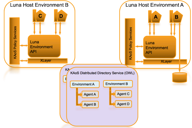
Figure 2: Luna Conceptual Architecture.
