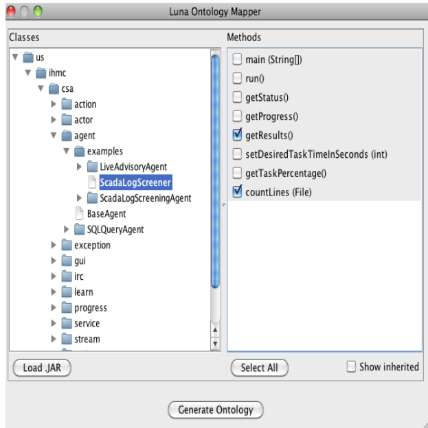
Figure 3: Java2OWL Tool.
